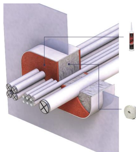
CABLES APPLICATION
