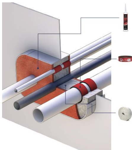
PIPES APPLICATION
